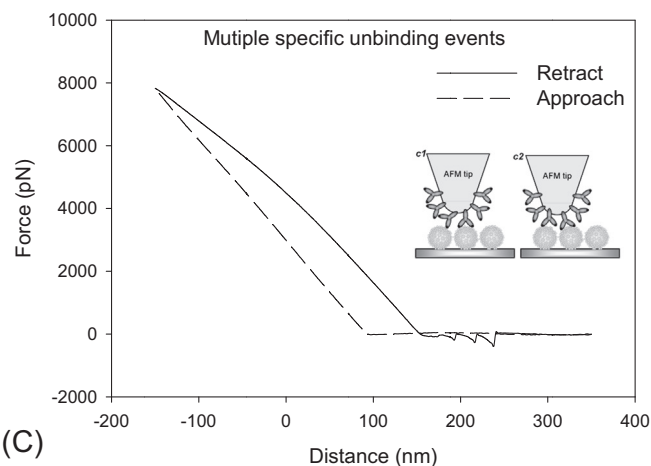
Fig. 3. Force-distance curves of the HPV16-anti-HPV16 L1 system with (A) mono-, (B) di, and (C) multi-unbinding events, which may be attributed to (A) a single, (B) sequential, and (C) multiple breaking of bond(s) between the substrate and the AFM tip. Schematic representations of the A, B, and C binding events are shown in a, b, and c, respectively. The HPV16 particles randomly immobilized on the substrate could be oriented (a1) or lying on the substrate (a2) with one binding site oriented to bind a single anti-HPV16 L1 on the AFM tip. Two separate anti-HPV16 L1 on the AFM tip can bind to two identical combining sites on one HPV16 (b1) or to separate combining sites on two HPV16 particles (b2). Several separate anti-HPV16 L1 molecules on the AFM tip can bind to three (c1) separate combining sites on HPV16 particles.
