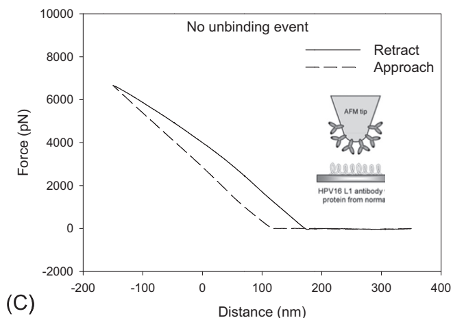
Fig. 2. Typical measurements of unbinding forces acquired by AFM contact mode. Force-distance curves of no adhesive force appeared during the retraction process, which were acquired by use of (A) AFM tip/glass and (C) HPV16 L1 antibody/protein from normal systems as two control experiments. (B) A representative force-distance curve of the HPV16-anti-HPV16 L1 system with a specific unbinding event which appeared during the retracting process.
